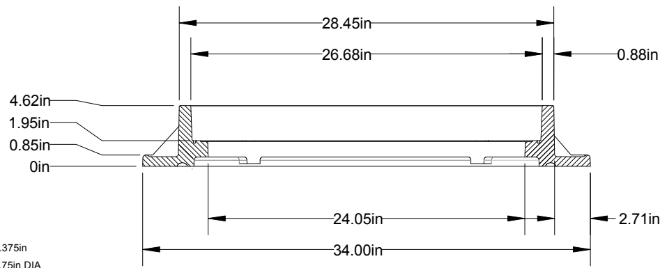
FRAME SECTION
