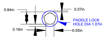
HOLE TO BOLT CLEARANCES
