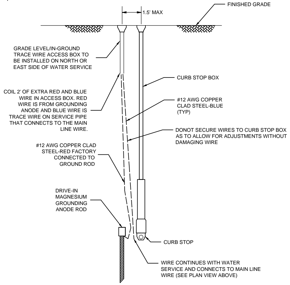
WATER SERVICE - SECTION VIEW NO SCALE
